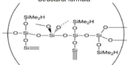
Structural formula
